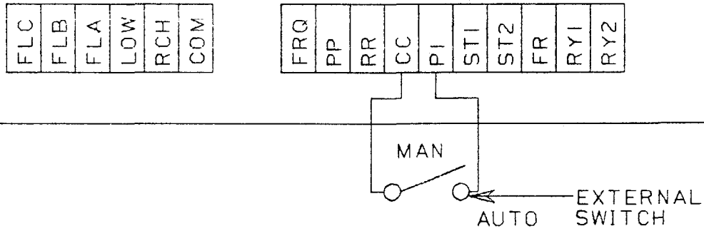
Figure 8A. MAN/AUTO Function Included
