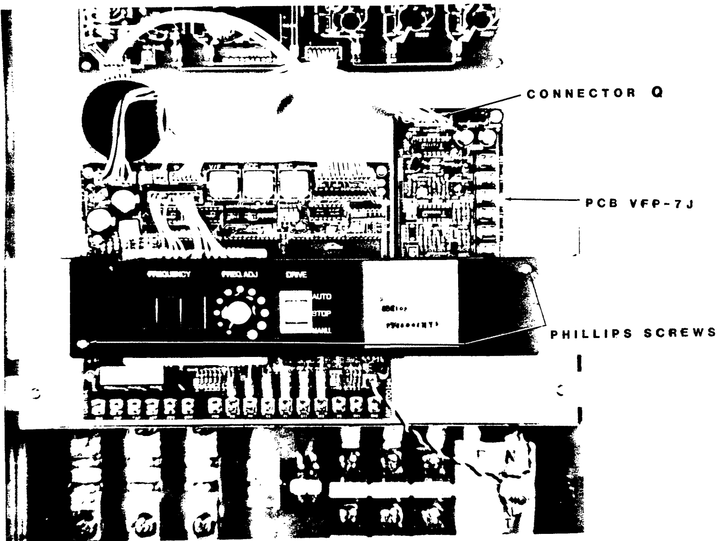
Figure 4. Component Location
