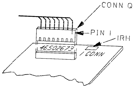
Figure 6. Connector Orientation
