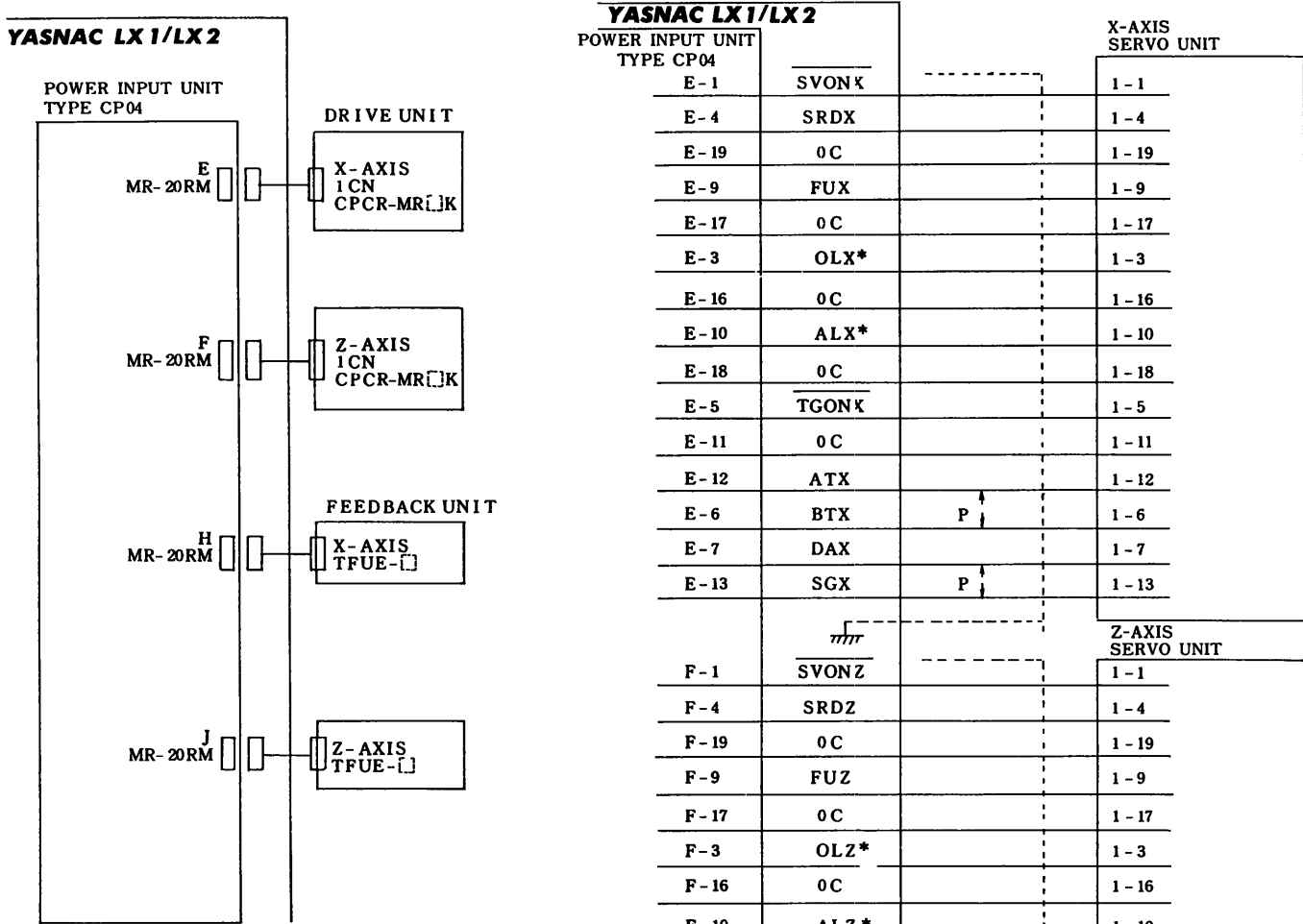
Fig 6 Wiring of Servopack and YASNAC LX1/LX2
